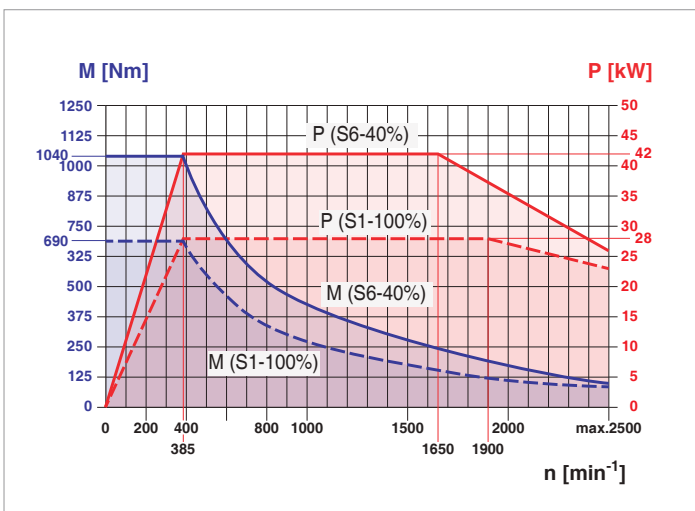
Performance and torque curve for main spindle with belt-drive
