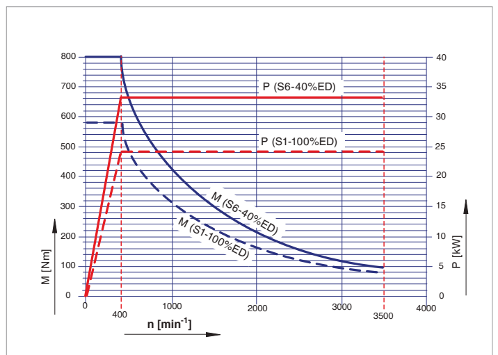
Performance and torque curve for main spindle with direct drive
