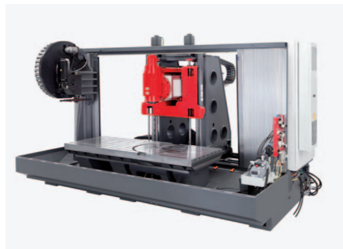
Machine frame. The machine frame is a polymer-concrete bed. This ensures the required rigidity of the machine base, and also facilitates vibration dampening.
