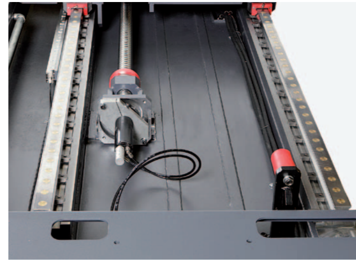
Axis drives. Linear axes are equipped with linear guides. Long way-guides are used to attain the necessary rigidity. The drive is equipped with a ball screw drive with direct drive bellows coupling. The direct drive provides for highly dynamic axis travel, while also employing a low maintenance and smooth drive system. The X-axis linear scale is standard due to the long travel.
