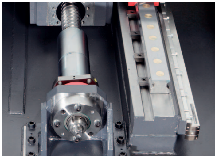
Glass scales. Due to its length, the X-axis is always equipped with glass scales. Y and Z axis can be equipped with glass scales on demand.
