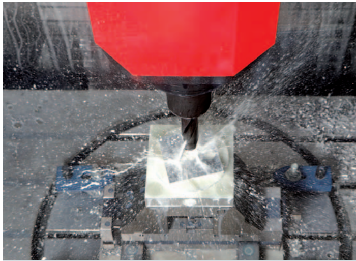
Coolant through the spindle. The spindle can be optionally flooded with high-pressure coolant (25 to 70 bar [362 to 1,015 psi]). This ensures reliable chip removal from holes and pockets and reduces cycle times for this type of machining.
