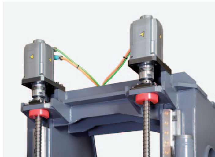
Z-axis travel. In order to attain precision Z-axis rapid travel at speeds of 50 m/min, and due to its large mass, this axis is powered by two ball screw drives and two motors in a master-slave configuration.
