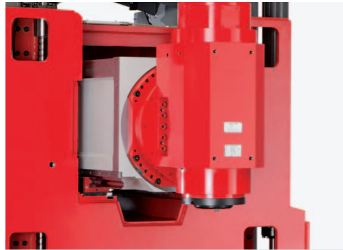
Milling spindle. The machine is equipped with a liquid cooled motor spindle with compelling performance specs. At spindle speeds of 15000 rpm, a power rating of 46 kW, and a torque of 170 Nm, the machine is also suited for heavy-duty machining. A motor spindle 18000 rpm is available with HSK A63.
