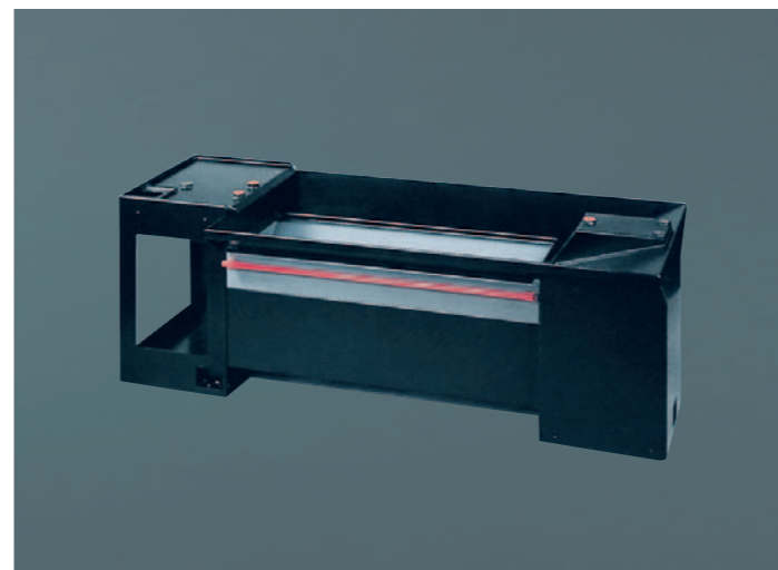
Machine stand. The machine stand absorbs vibrations. Slanted collection plates make cleaning easy and allow coolant to drain quickly.
