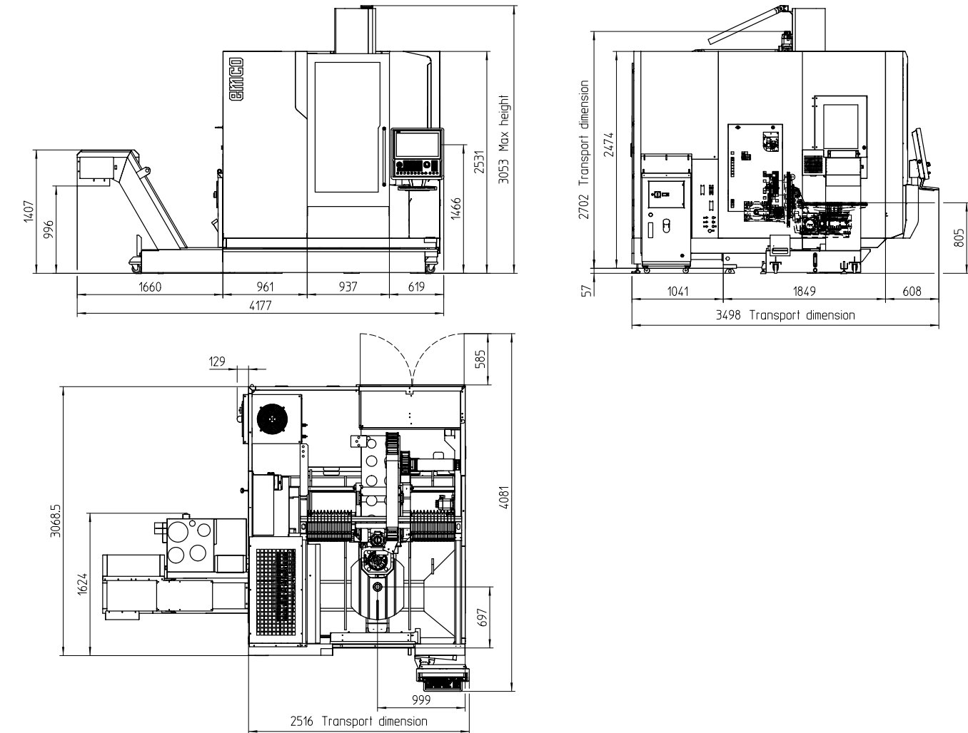
MAXXMILL 750
