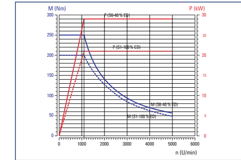
Main and counter spindle Ø 65 mm / Ø 76 mm
