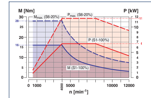
Tool turret with direct drive - BMT55P
