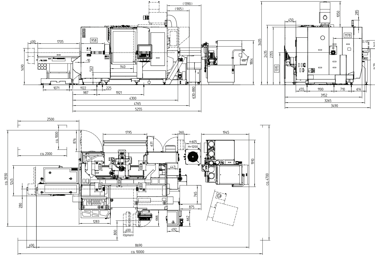
Installation plan HT65 PM HP
