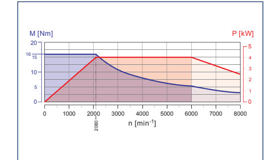
Characteristic of driven tools MT45-HSC tool turret
