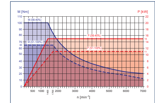
Main spindle / counter spindle motor characteristics
