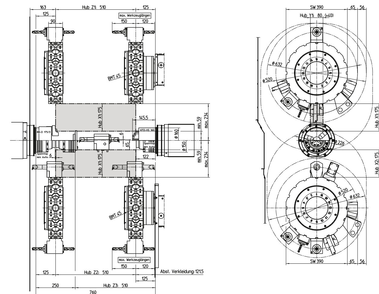
Work area HT50 with 16-station BMT45P turret
