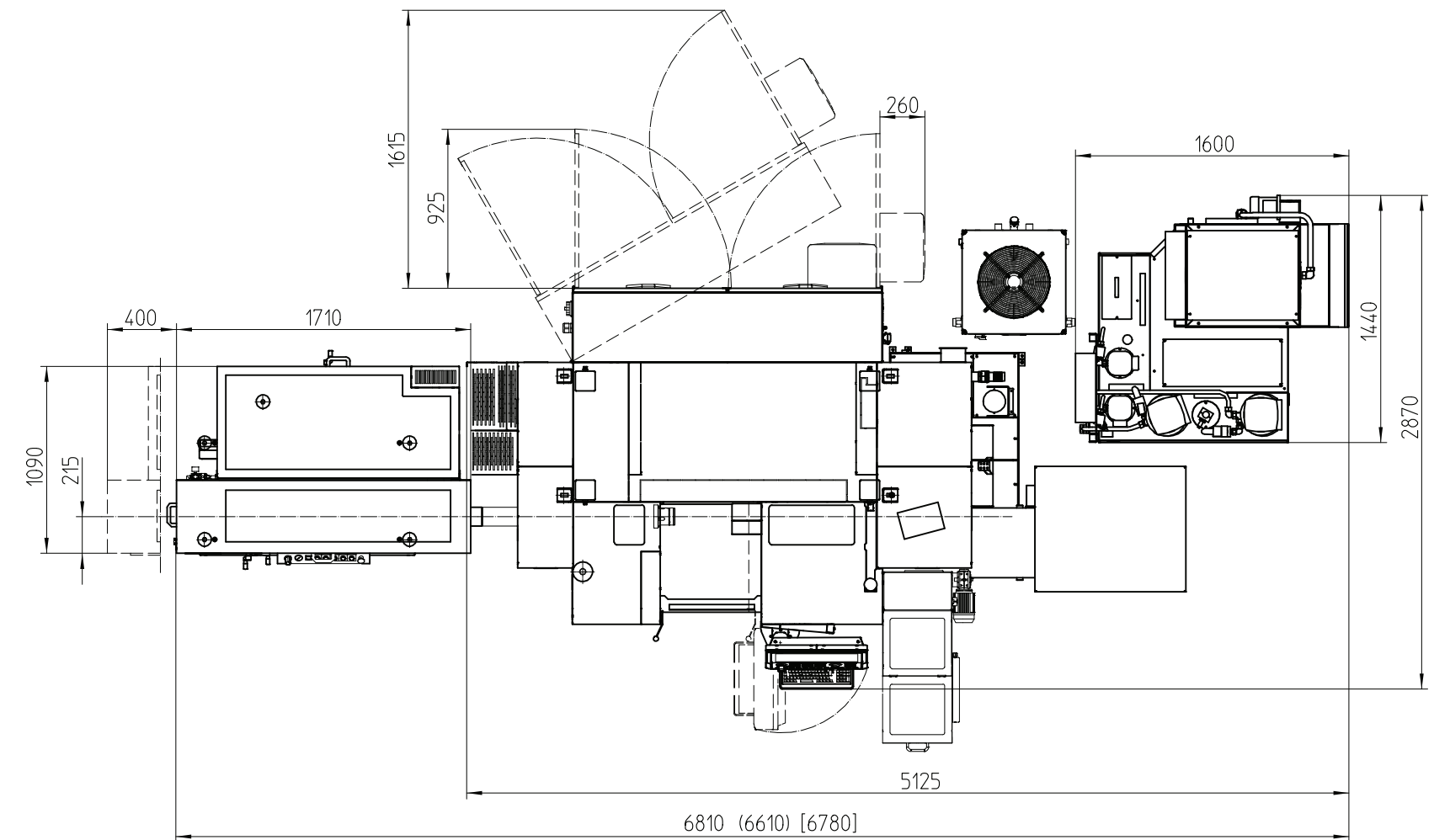
Floor plan HT50 with EMCO SL 1200 and paper band filter system
