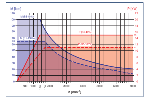
HYPERTURN 50 main spindle / counter spindle
