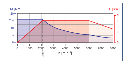
VDI25 tool turret with driven tools
