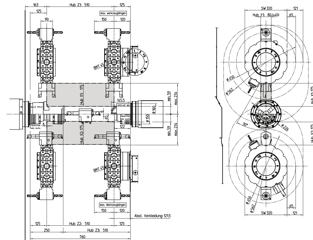
Work area HT50 with 12-station BMT45P turret
