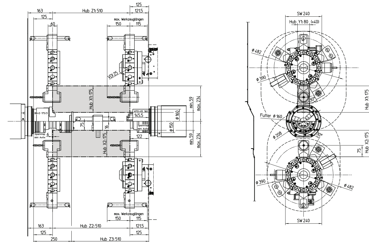
Work area HT50 with 12-station VDI 25 turret
