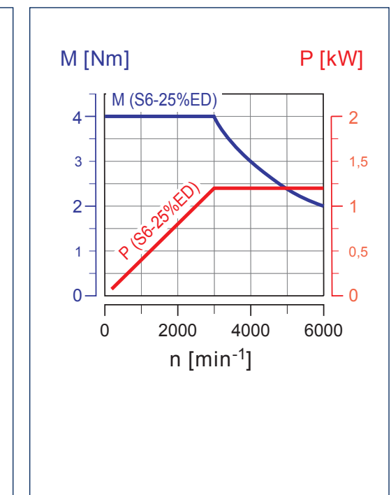
Motor characteristic curve tool turret (driven tools)
