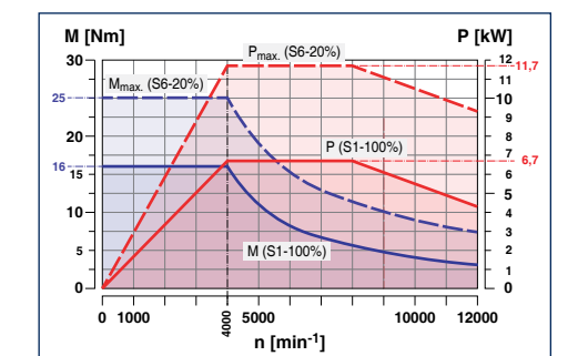
Tool turret with direct drive - BMT45P
